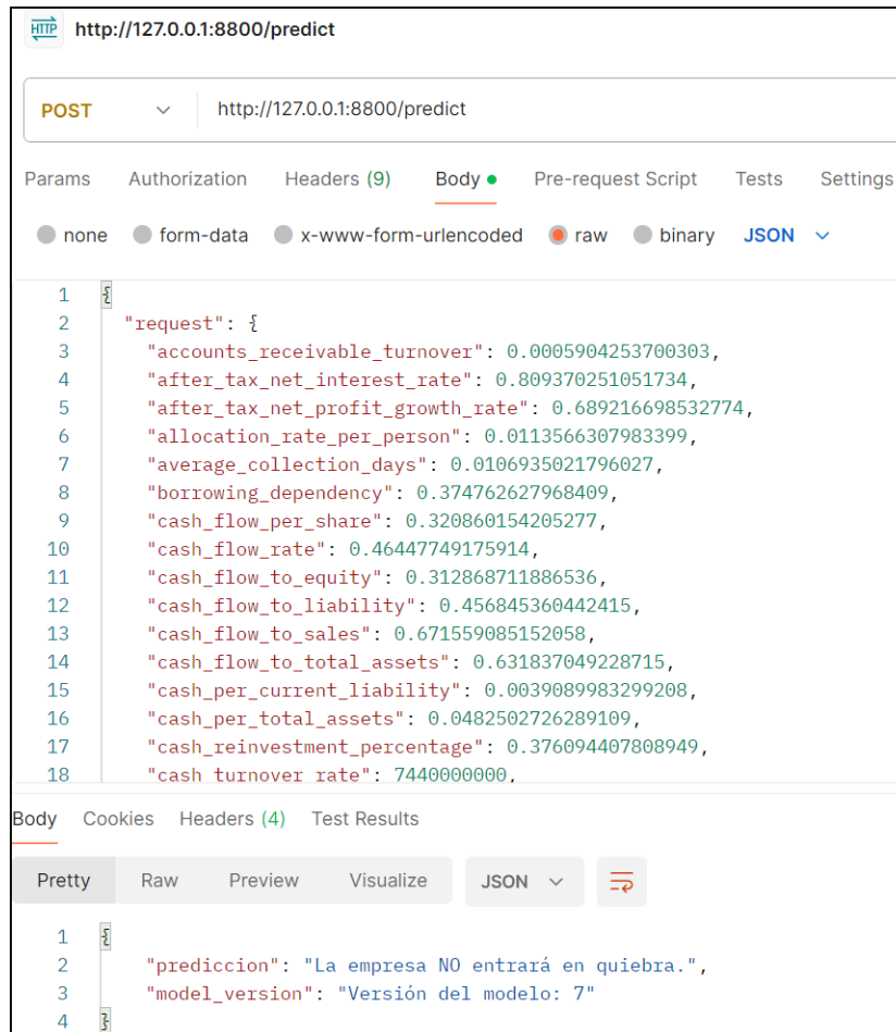
FIGURA 4.9. Endpoint predict
